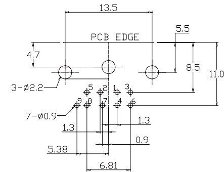
P.C.B. RECOMMEND LAYOUT BOTTOM VIEW
